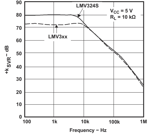
Figure 6-20. +k_{SVR} vs Frequency
