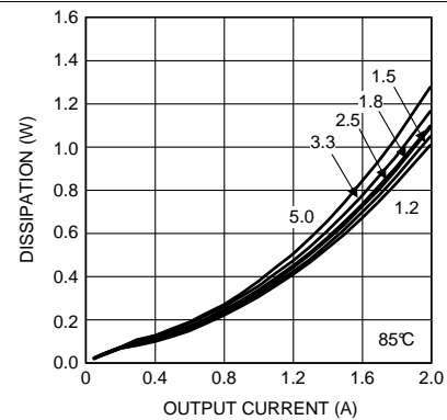
Figure 14. Dissipation 8-V Input at 85°C
