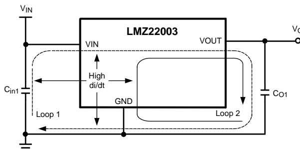
Figure 52. Critical Current Loops to Minimize
