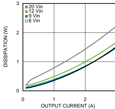
Figure 10. Dissipation 1.8-V Output at 25°C Ambient
