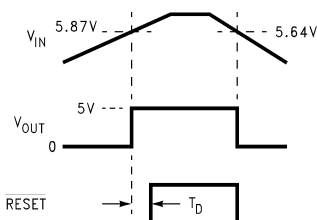
Figure 42. Timing Diagram
