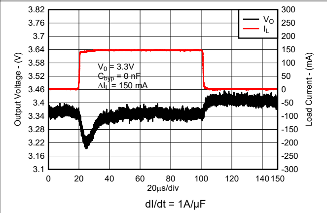
Figure 7-13. Load Transient Response (New Chip)
