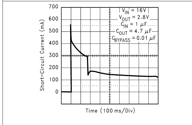
Figure 7-6. Short-Circuit Current (Legacy Chip) at V_{IN} = 16\text{V}
