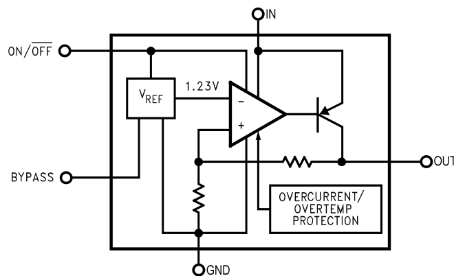
Figure 6-1. Block Diagram for Legacy Chip
