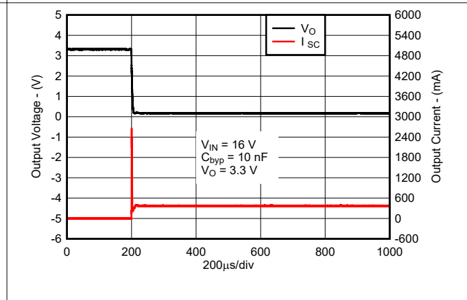
Figure 7-7. Short-Circuit Current (New Chip) at V_{IN} = 16\text{V}
