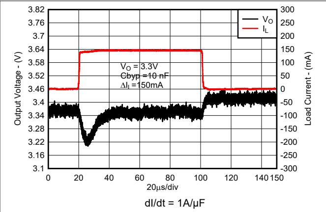
Figure 7-11. Load Transient (New Chip)
