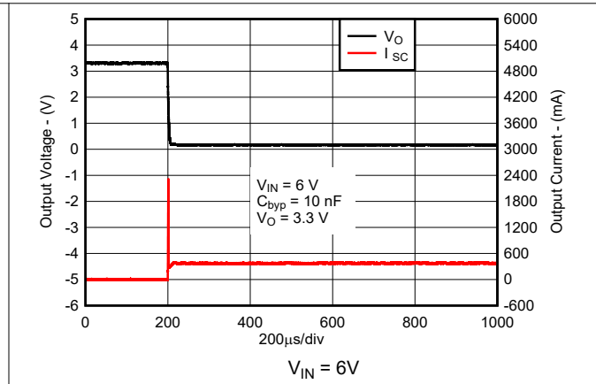
Figure 7-5. Short-Circuit Current (New Chip) at V_{IN} = 6\text{V}
