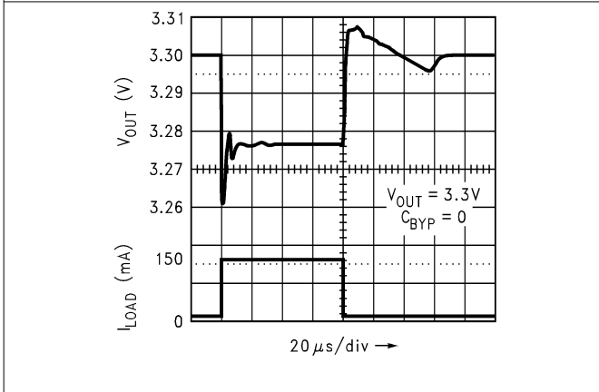
Figure 7-12. Load Transient Response (Legacy Chip)
