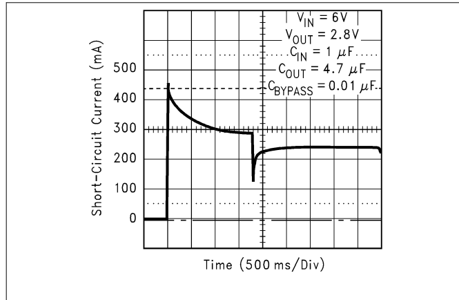
Figure 7-4. Short-Circuit Current (Legacy Chip) at V_{IN} = 6\text{V}
