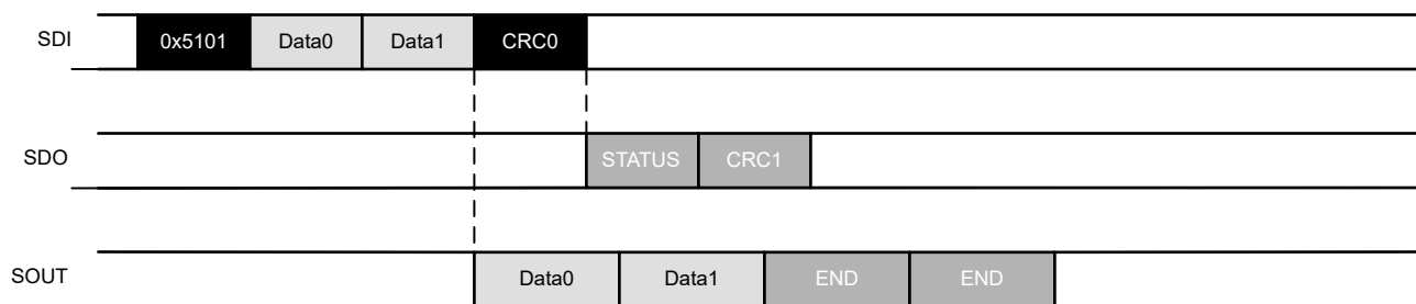
Figure 7-12. Example of FWD_WR_END command
