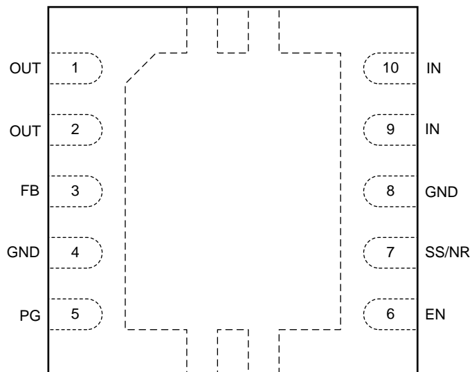
DSC Package 10-Pin WSON With Thermal Pad Top View
