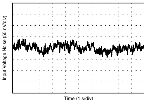
OPAx210 0.1-Hz to 10-Hz Noise
