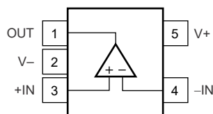
Figure 5-1. OPA620: DBV Package, 5-Pin SOT-23 (Top View)
