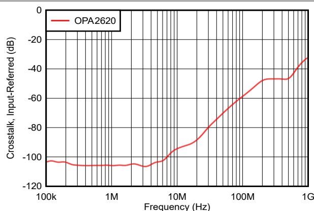
Figure 6-27. Channel-to-channel crosstalk
