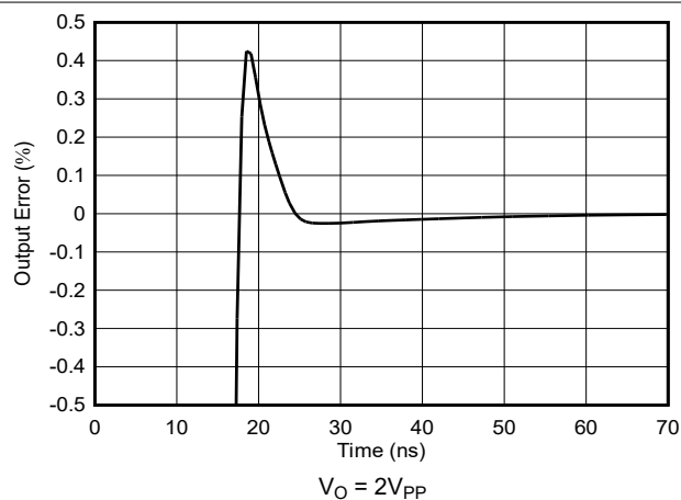
Figure 6-23. Output Settling Time to 0.1%
