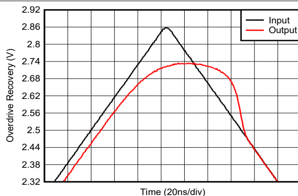
Figure 6-28. Overdrive Recovery
