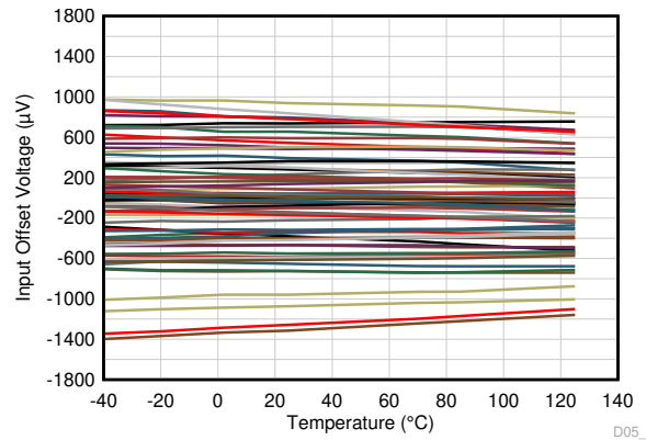
Figure 5-8. Input Offset Voltage vs Temperature
