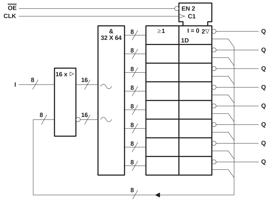
PAL16R8AM PAL16R8A-2M
