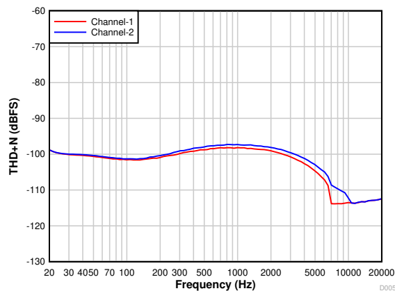
Figure 7-3. PCM1820: THD+N vs Input Frequency With a -60\text{-dBr} Input
