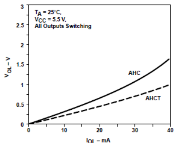
Figure 8-3. AHC Family V_{OL} vs I_{OL}
