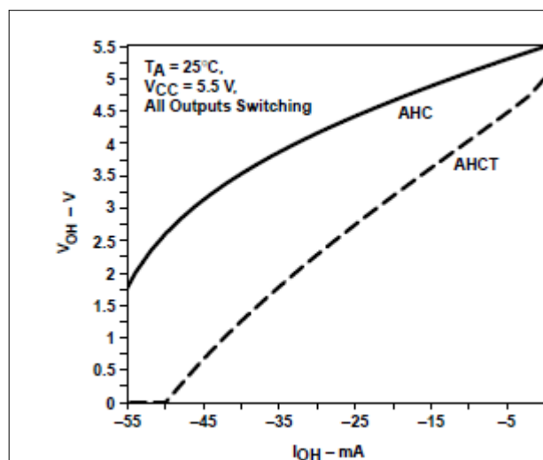
Figure 8-2. AHC Family V_{OH} vs I_{OH}
