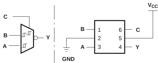
Figure 5. 157+04: 2-to-1 Data Selector With Inverted Output When C is L, Y = \overline{B} When C is H, Y = \overline{A}
