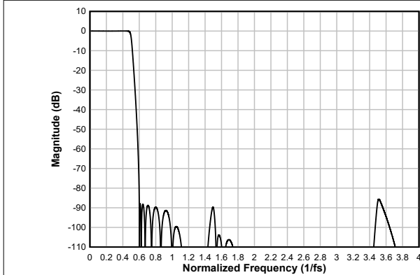
Figure 6-46. Low-latency Decimation Filter Magnitude Response
