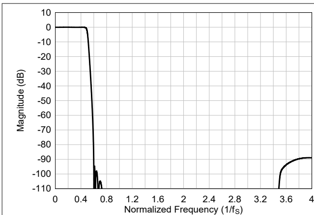
Figure 6-89. Ultra-Low-Latency interpolation Filter Magnitude Response
