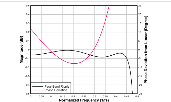
Figure 6-90. Ultra-Low-Latency interpolation Filter Pass-Band Ripple and Phase Deviation
