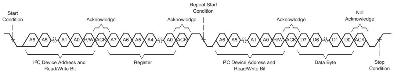
Figure 6-100. I 2 C Single-Byte Read Transfer
