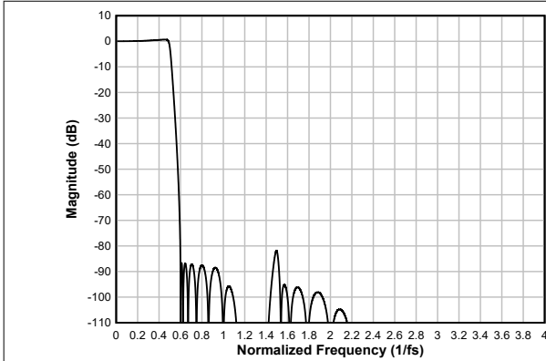
Figure 6-40. Low-latency Decimation Filter Magnitude Response
