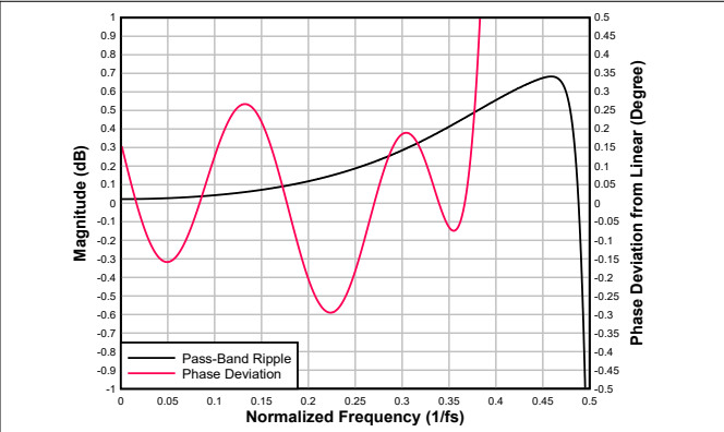
Figure 6-41. Low-latency Decimation Filter Pass-Band Ripple and Phase Deviation
