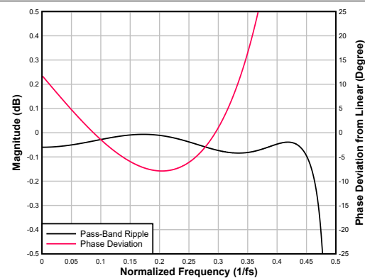
Figure 6-92. Ultra-Low-Latency interpolation Filter Pass-Band Ripple and Phase Deviation
