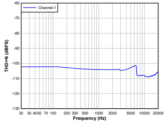
Differential receiver output, 32Ω load (-1dBFS input)
