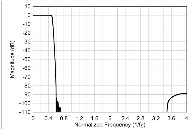
Figure 6-87. Ultra-Low-Latency interpolation Filter Magnitude Response
