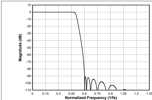
Figure 6-48. Low-latency Decimation Filter Magnitude Response
