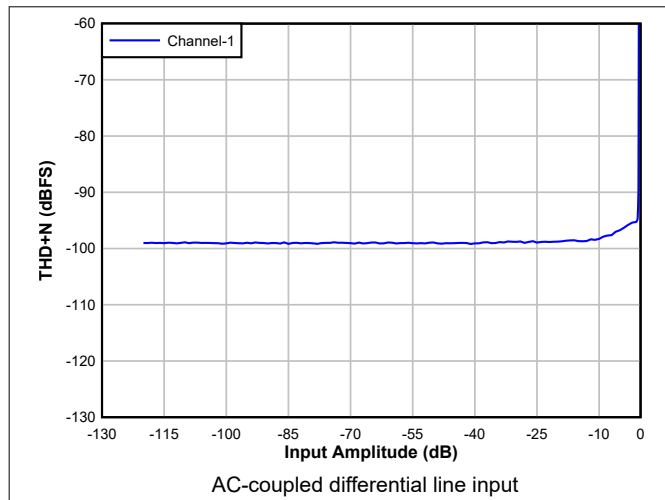
Figure 8-2. ADC THD+N Level vs Input
