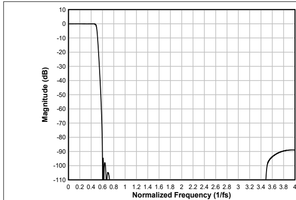
Figure 6-77. Low-latency Interpolation Filter Magnitude Response
