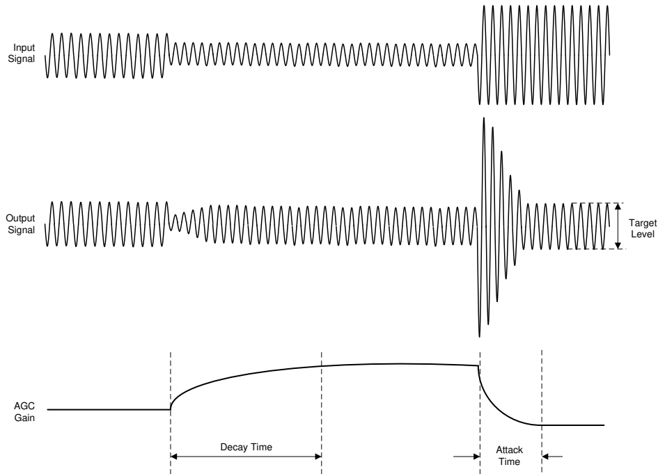
Figure 6-60. AGC Characteristics
