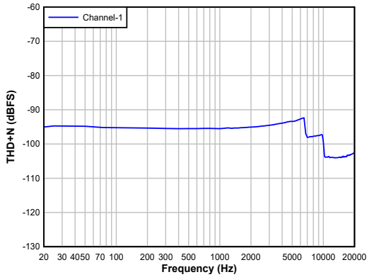
Single-ended output (-1dBFS input)
