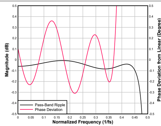
Figure 6-78. Low-latency Interpolation Filter Pass-Band Ripple and Phase Deviation
