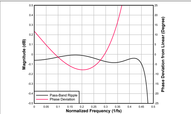
Figure 6-88. Ultra-Low-Latency interpolation Filter Pass-Band Ripple and Phase Deviation
