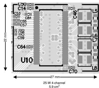
PCB AREA
