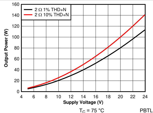
Figure 7-32. Output Power vs Supply Voltage - PBTL
