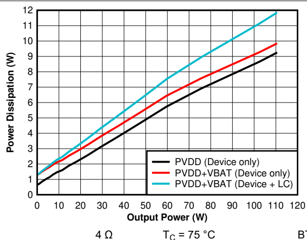
Figure 7-24. Power Dissipation vs Output Power - 4 \Omega - 384 kHz
