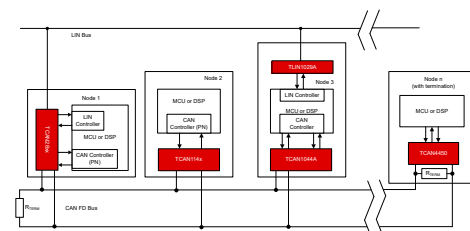
Simplified Schematic
