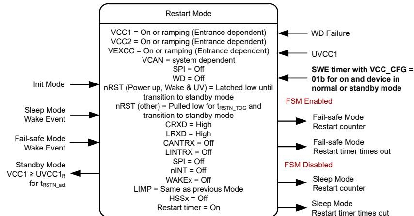
Figure 8-24. Restart Mode
