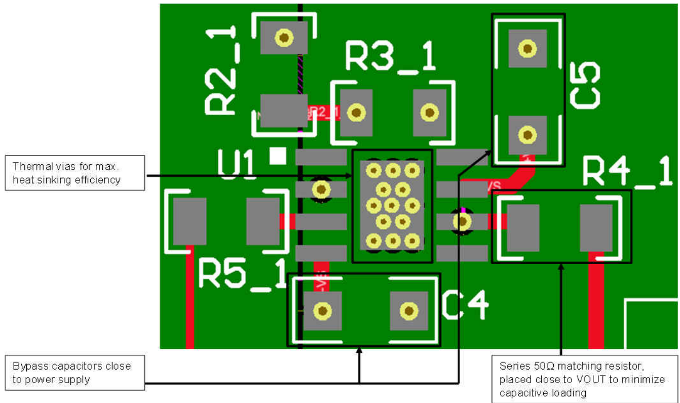
Figure 9-8. Layout Recommendation
