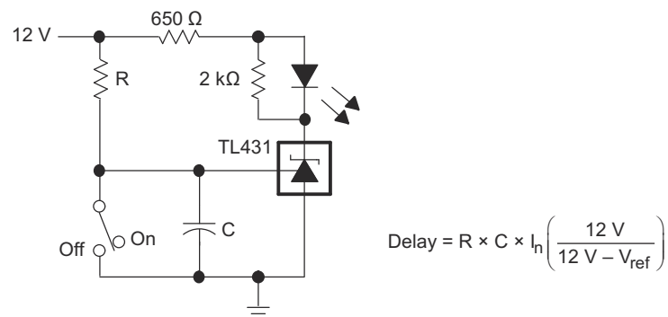
Figure 9-13. Delay Timer
