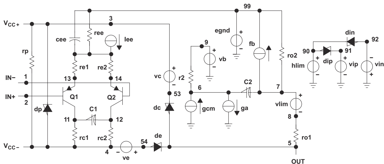
Figure 8-3. Boyle Subcircuit
