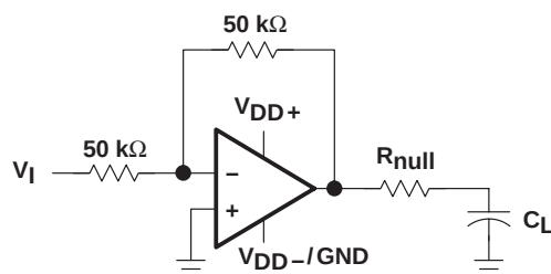
Figure 60. Series-Resistance Circuit
