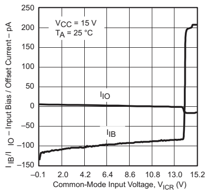
Figure 9. Input Bias and Offset Current vs Common-Mode Input Voltage
