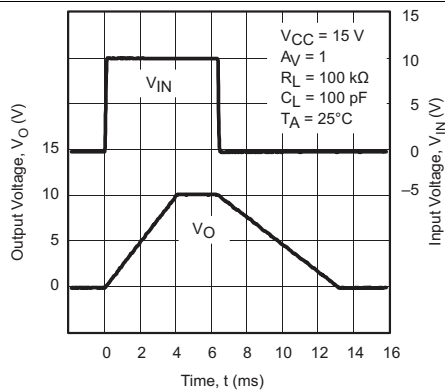
Figure 30. Large Signal Follower Pulse Response
