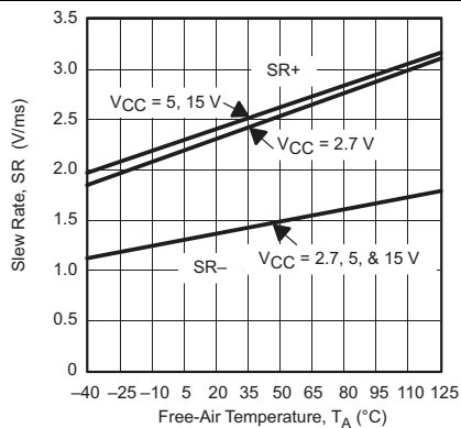
Figure 23. Slew Rate vs Free-Air Temperature
