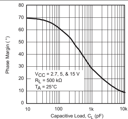
Figure 24. Phase Margin vs Capacitive Load
