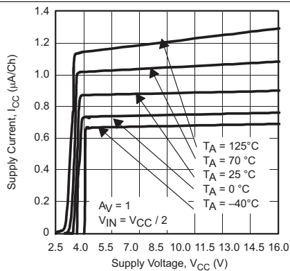
Figure 19. Supply Current vs Supply Voltage
