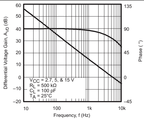
Figure 21. Differential Voltage Gain and Phase vs Frequency
