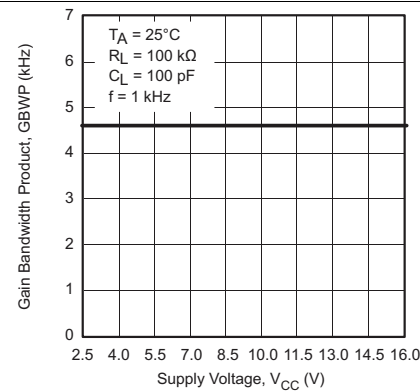
Figure 22. Gain Bandwidth Product vs Supply Voltage
