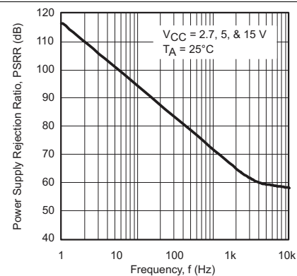
Figure 20. Power Supply Rejection Ratio vs Frequency
