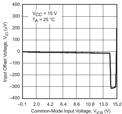
Figure 3. Input Offset Voltage vs Common-Mode Input Voltage
