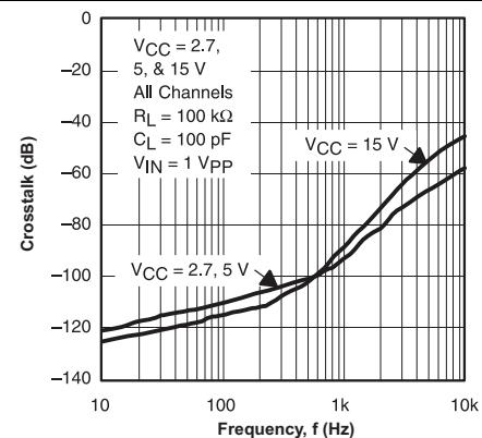
Figure 36. Crosstalk
