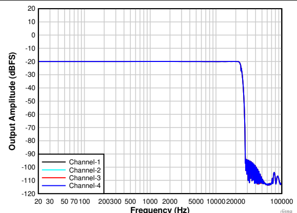
Figure 7-27. PDM Input Frequency Response With a -20-dBr Input
