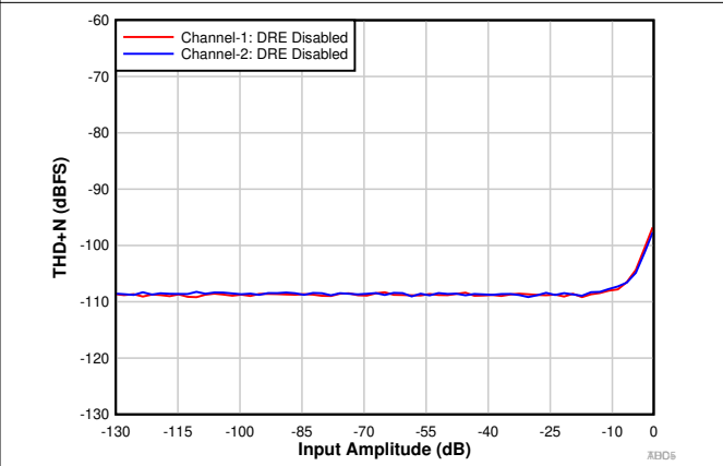
Figure 9-5. THD+N vs Input Amplitude With DRE Disabled
