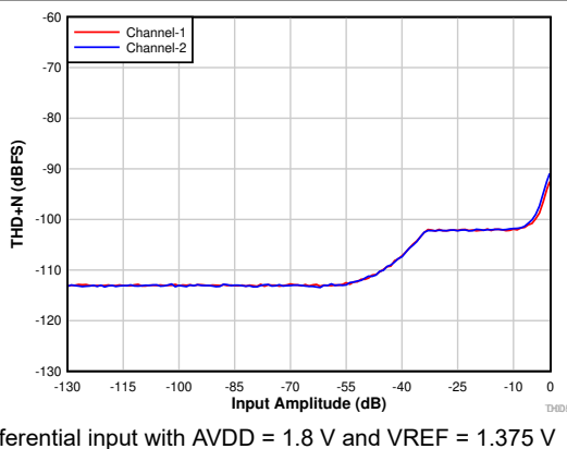
Differential input with AVDD = 1.8\text{ V} and VREF = 1.375\text{ V} Figure 7-8. THD+N vs Input Amplitude With DRE Enabled
