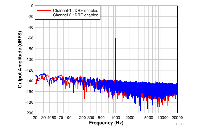
Figure 9-2. FFT With a –60-dBr Input With DRE Enabled
