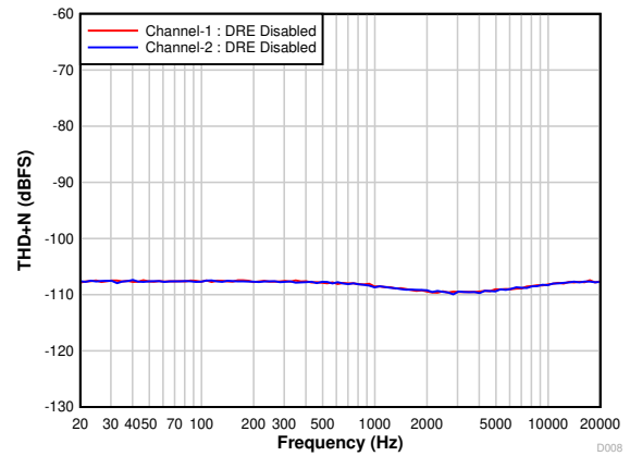
Figure 7-11. THD+N vs Input Frequency With a -60-dBr Input
