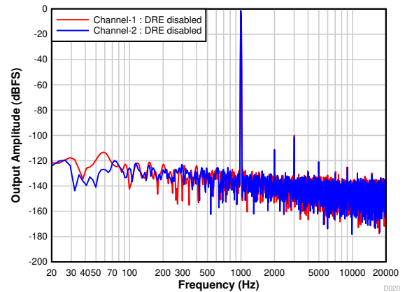
Figure 7-23. FFT With a -1-dBr Input With DRE Disabled
