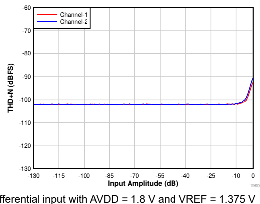
Differential input with AVDD = 1.8\text{ V} and VREF = 1.375\text{ V} Figure 7-9. THD+N vs Input Amplitude With DRE Disabled
