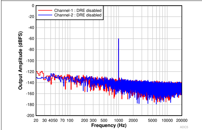
Figure 9-4. FFT With a –60-dBr Input With DRE Disabled
