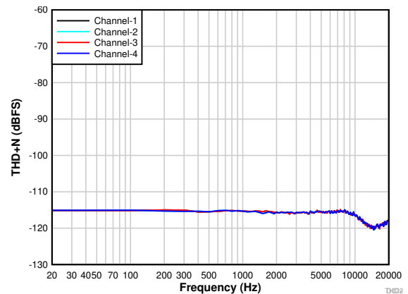
Figure 7-25. PDM Input THD+N vs Input Frequency With a -20-dBr Input
