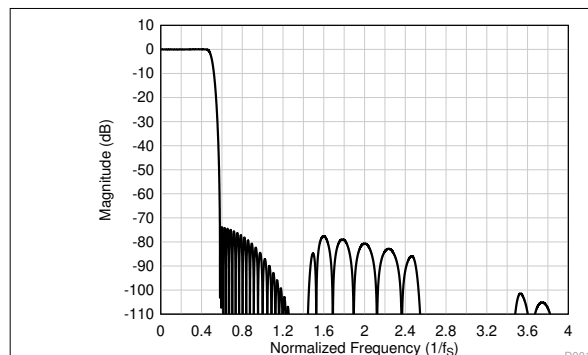
Figure 8-25. Linear Phase Decimation Filter Magnitude Response
