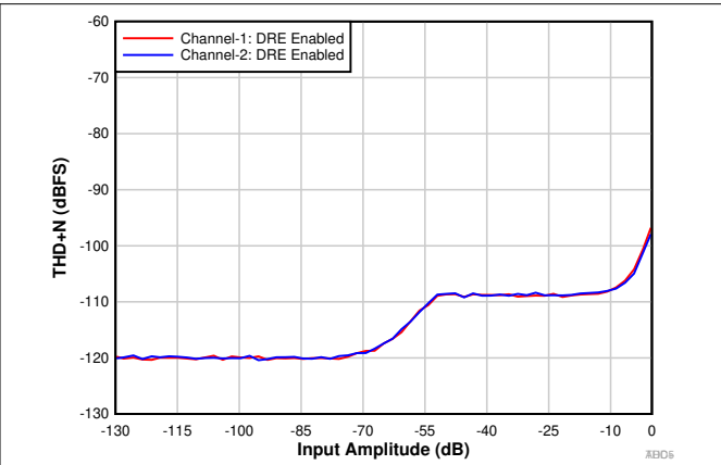
Figure 9-3. THD+N vs Input Amplitude With DRE Enabled
