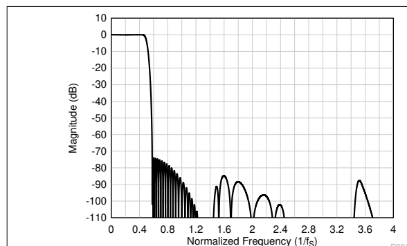
Figure 8-27. Linear Phase Decimation Filter Magnitude Response
