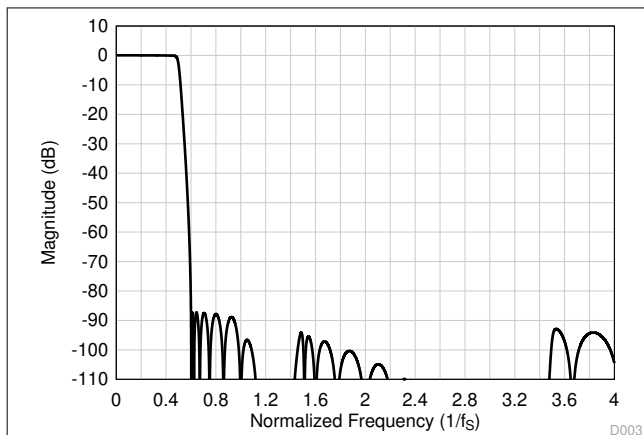
Figure 8-49. Ultra-Low-Latency Decimation Filter Magnitude Response
