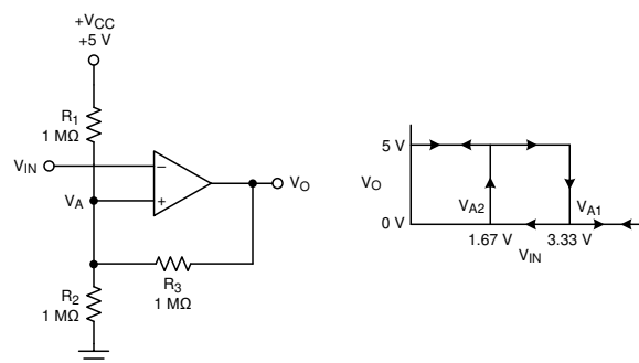
Figure 7-3. TLV3511 in an Inverting Configuration With Hysteresis
