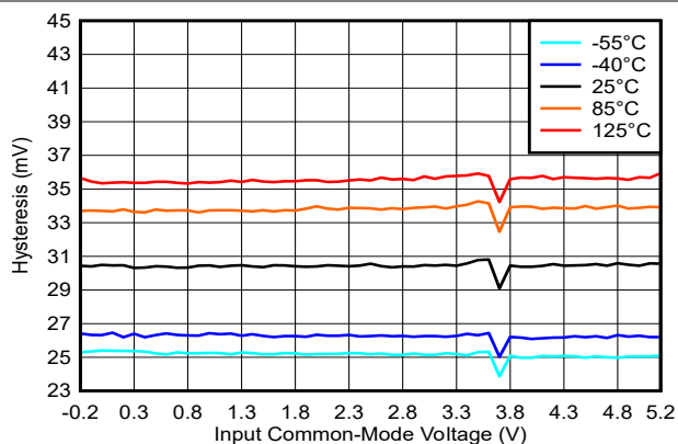
Figure 5-10. Hysteresis vs. Common-Mode, 5V
