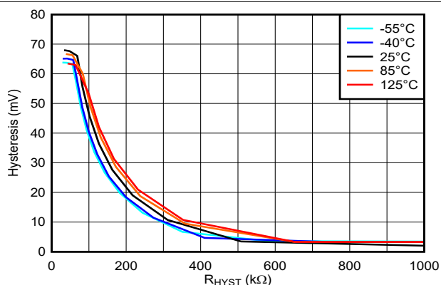
Figure 5-12. Hysteresis vs. Resistance, 3.3V
