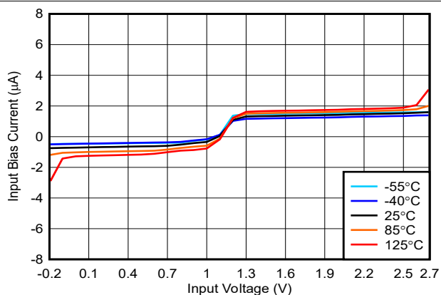
Figure 5-14. Bias Current vs. Input Voltage, 2.5V
