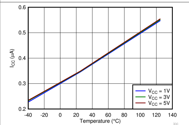
Figure 5-26. I_{CC} vs Temperature
