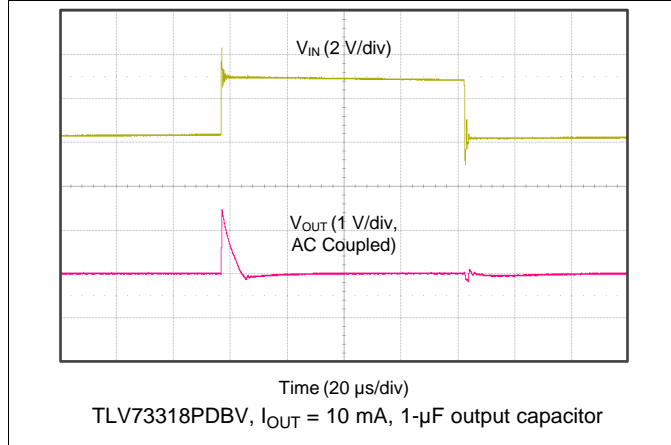
Figure 23. Line Transient
