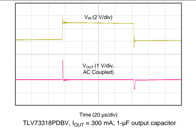
Figure 24. Line Transient
