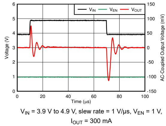
Figure 5-20. Line Transient
