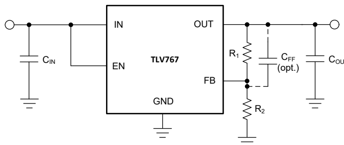
Figure 9-2. Typical Application Circuit
