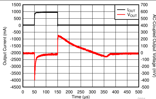
Figure 7-11. I_{OUT} Transient From 1\text{ mA} to 1\text{ A}
