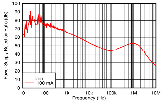
Figure 9-4. PSRR Performance
