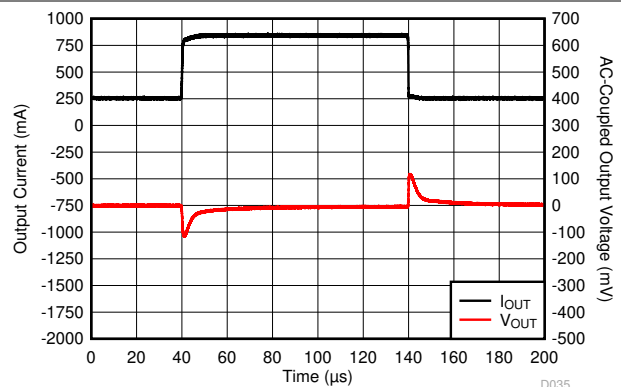
Figure 7-12. I_{OUT} Transient From 250\text{ mA} to 850\text{ mA}
