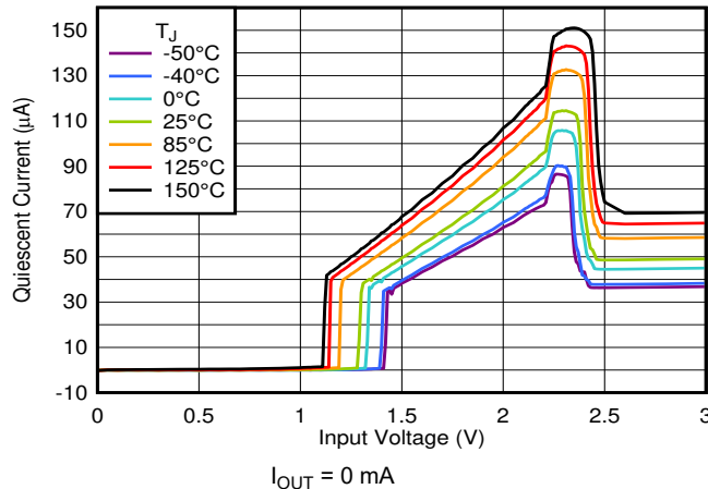
Figure 7-9. I_Q Increase Below Minimum V_{IN}
