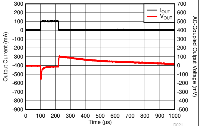
Figure 7-10. I_{OUT} Transient From 0\text{ mA} to 100\text{ mA}
