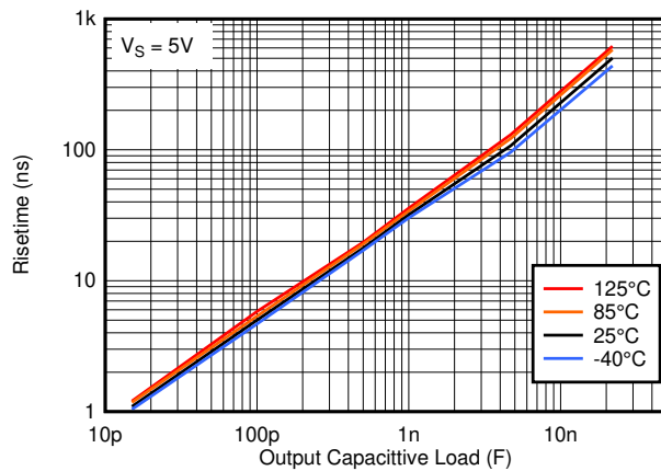
Figure 5-15. Risettime vs Capacitive Load
