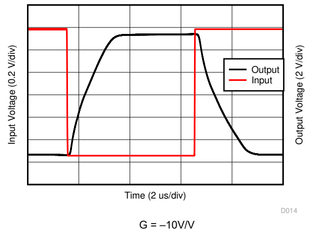
Figure 6-22. Overload Recovery
