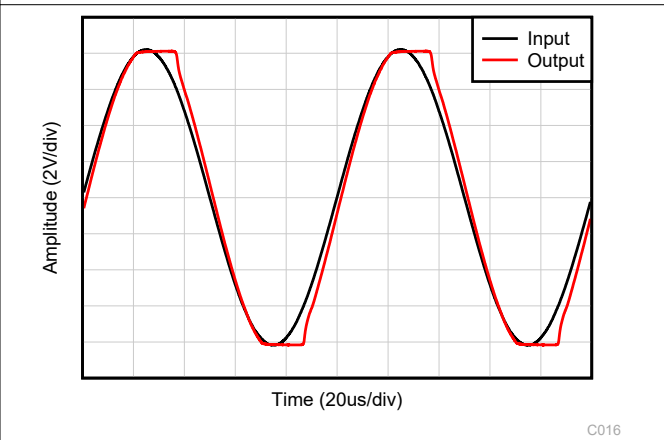
Figure 6-30. No Phase Reversal V_{IN} = \pm 8\text{ V} ; V_S = V_{OUT} = \pm 17\text{ V}
