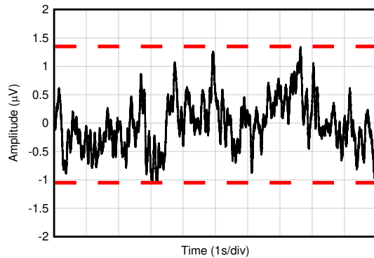
Figure 5-25. 0.1Hz to 10Hz Noise
