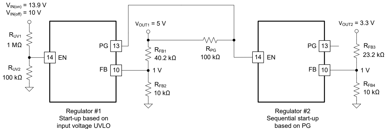
Figure 8-4. TLVM13620 Sequencing Implementation Using PG and EN
