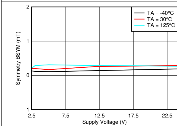
Figure 7-23. B_{SYM(Y)} vs. V_{CC}
