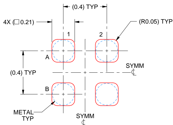
SOLDER PASTE EXAMPLE BASED ON 0.075 mm THICK STENCIL SCALE: 50X
