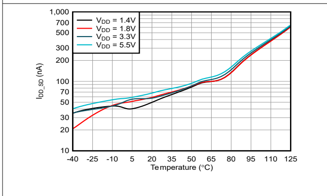
Figure 6-18. Shutdown Current vs Temperature
