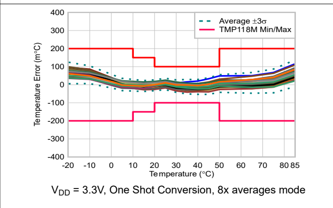
Figure 6-5. TMP118M Temperature Error vs Temperature
