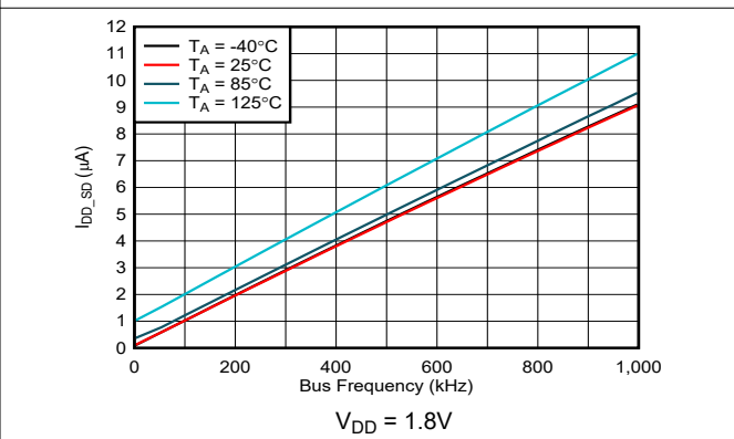
Figure 6-19. Shutdown Current vs Bus Frequency
