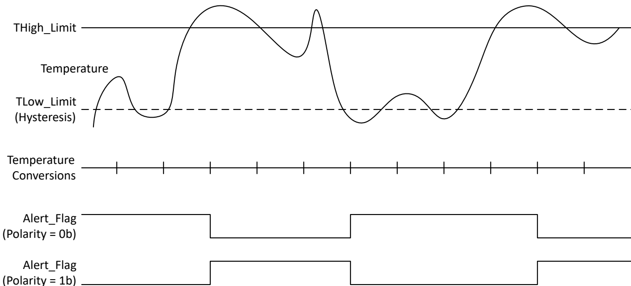
Figure 7-5. Alert_Flag Behavior
