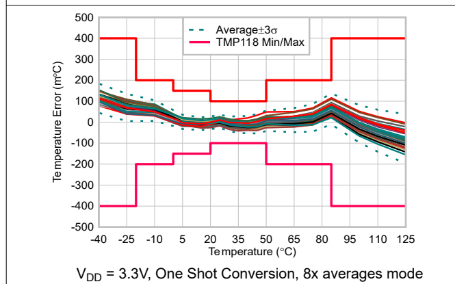
Figure 6-4. TMP118 Temperature Error vs Temperature
