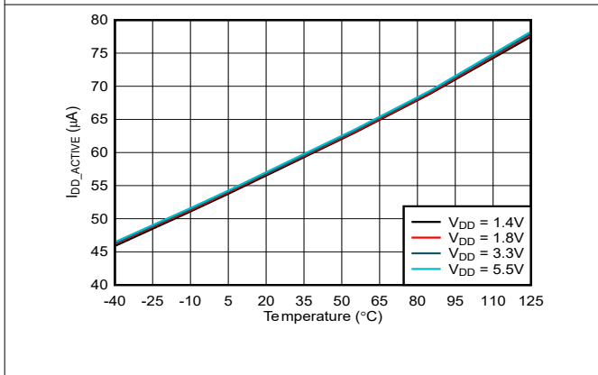
Figure 6-16. Active Conversion Current vs Temperature
