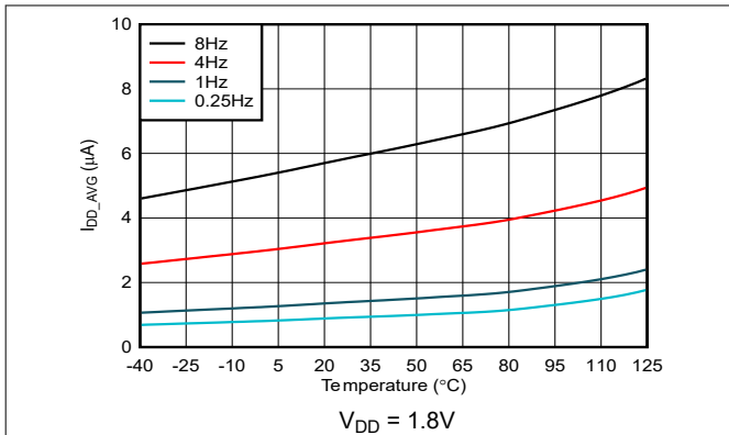
Figure 6-14. Average Quiescent Current vs Temperature
