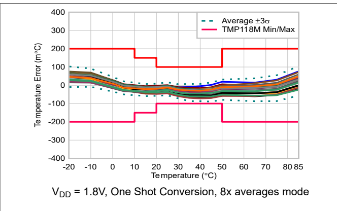
Figure 6-3. TMP118M Temperature Error vs Temperature
