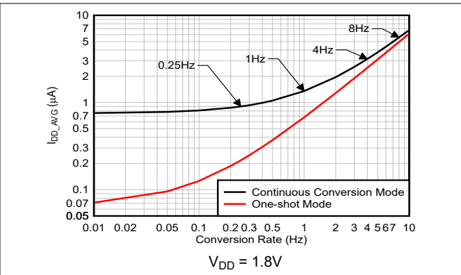
Figure 6-15. Average Quiescent Current vs Conversion Rate
