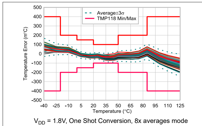
Figure 6-2. TMP118 Temperature Error vs Temperature
