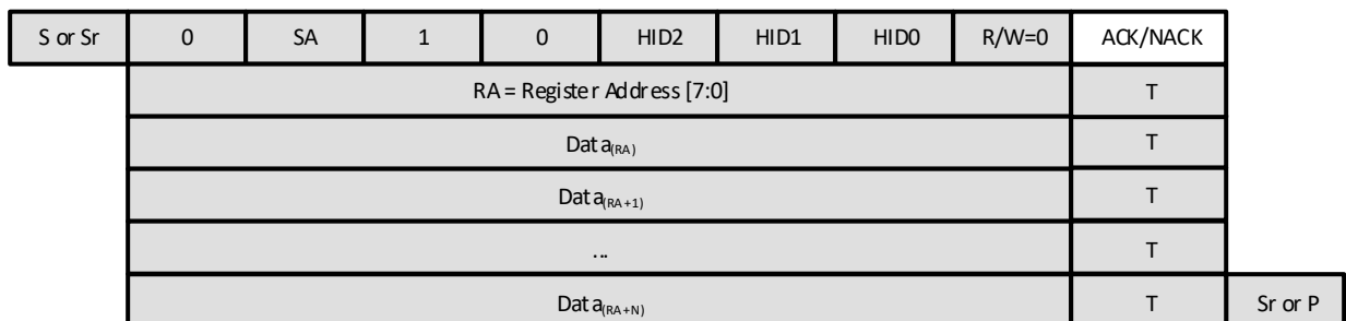
Figure 7-11. I3C Basic Mode Write
