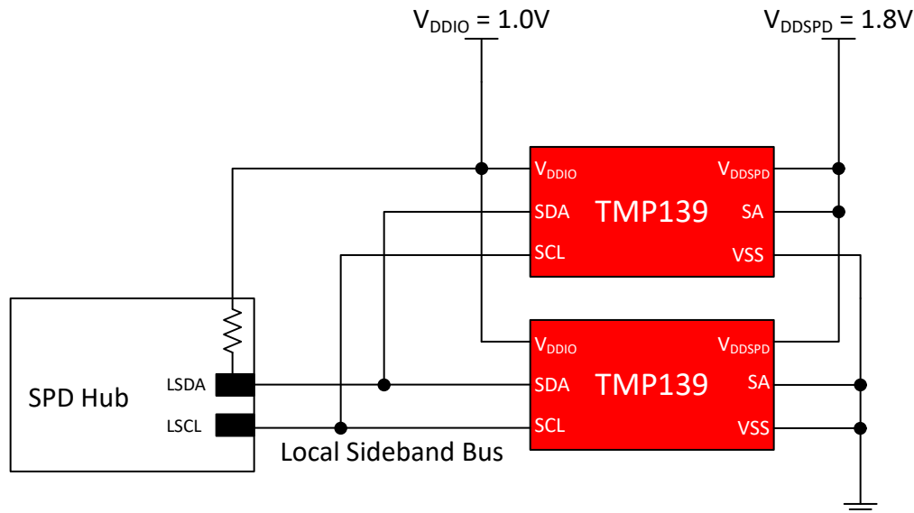
Figure 8-1. Typical Connections
