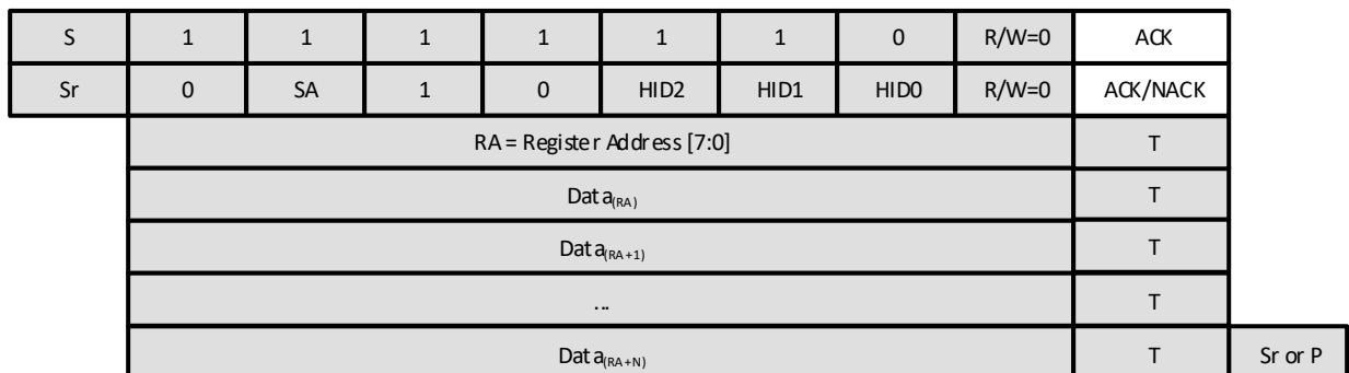
Figure 7-12. I3C Basic Mode Write with IBI Header
