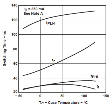
Figure 5-6. Switching Time vs Case Temperature
