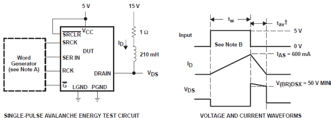
Figure 6-5. Reverse-Recovery-Current Test Circuit and Waveforms of Source-Drain Diode
