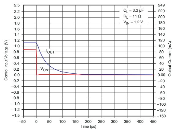
Figure 7-32. t OFF Response
