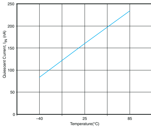
Figure 7-5. Quiescent Current vs Temperature ( V_{IN} = 3.3 V, I_{OUT} = 0 )
