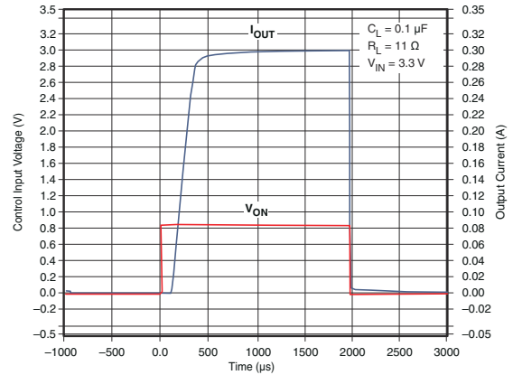
Figure 7-42. t_{ON} Response
