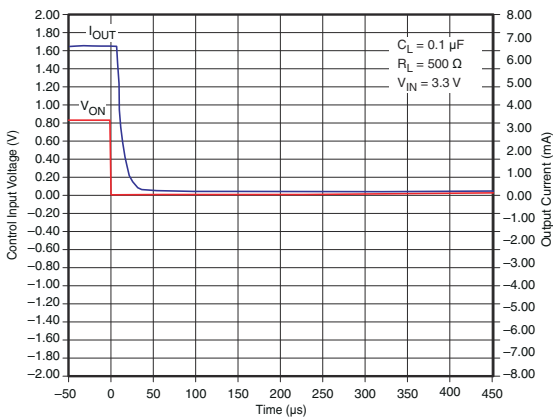
Figure 7-33. t OFF Response
