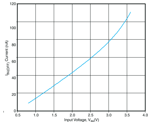
Figure 7-6. I_{IN(OFF)} vs V_{IN} ( V_{ON} = 0 V)
