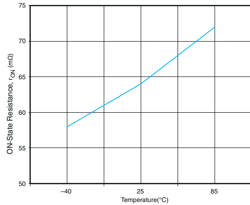
Figure 7-2. r_{ON} vs Temperature ( V_{IN} = 3.3 V)
