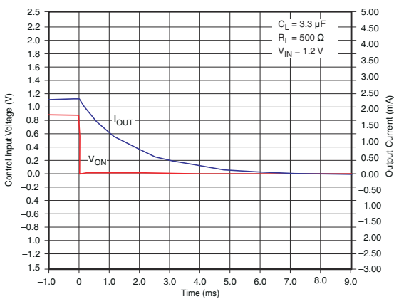
Figure 7-31. t OFF Response
