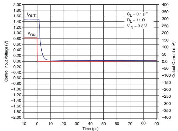
Figure 7-34. t OFF Response
