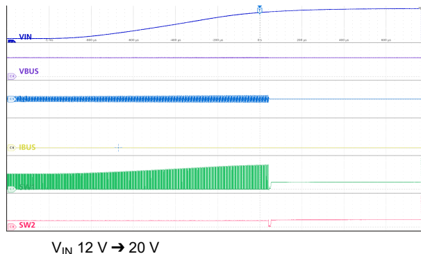
Figure 9-27. V_{IN(OVP)} Entry
