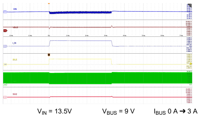
Figure 9-31. Load Transient (Buck): V_{BUS} = 9\text{ V}
