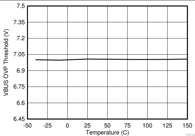
Figure 8-18. VBUS Overvoltage Protection Threshold vs Junction Temperature
