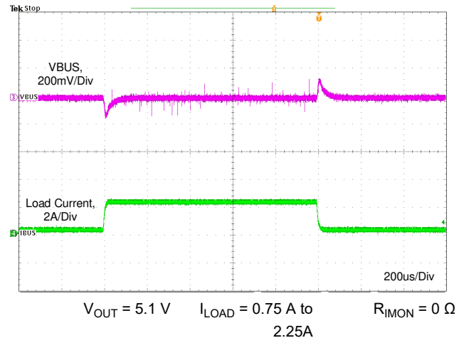
Figure 11-9. Load Transient Without Cable Compensation
