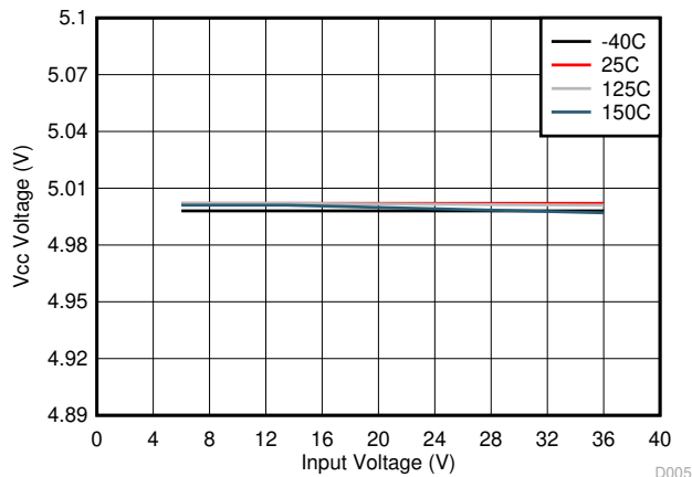
Figure 8-5. VCC vs Input Voltage
