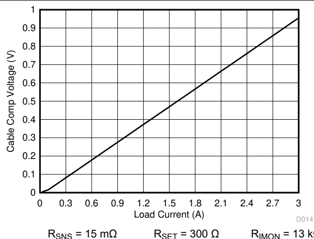
Figure 8-17. Cable Compensation Voltage vs Load Current
