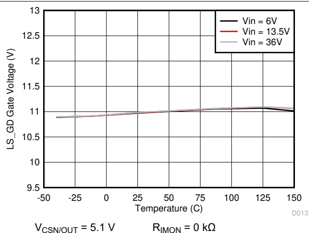
Figure 8-15. LS_GD Gate Voltage vs Junction Temperature
