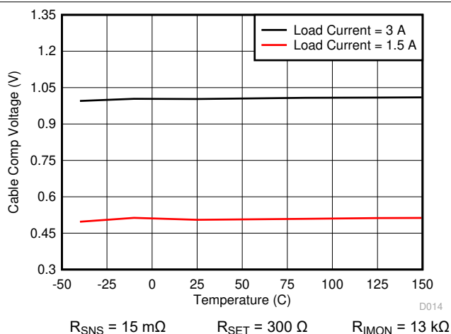
Figure 8-16. Cable Compensation Voltage vs Junction Temperature
