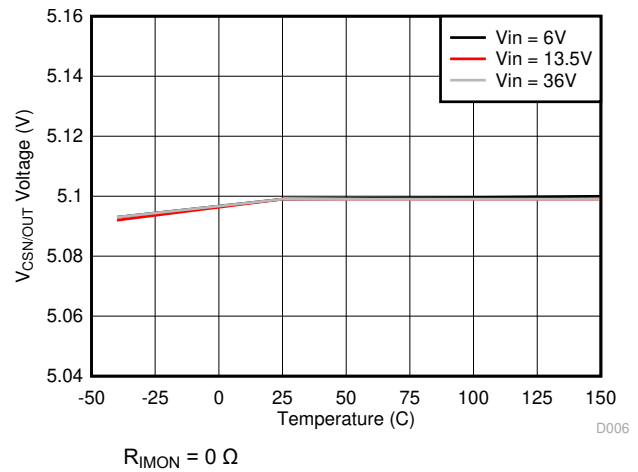
Figure 8-6. V_{CSN/OUT} Voltage vs Junction Temperature
