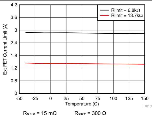
Figure 8-13. External FET Current Limit vs Junction Temperature
