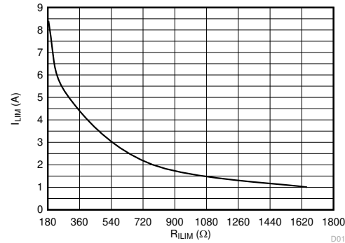
Figure 7-10. Output Current Limit ( I_{LIM} ) vs R_{LIM}
