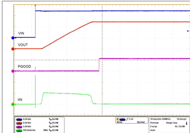
A. C_{OUT} = 1.4\text{mF} C_{dVdt} = 10\text{nF} R_{L(SU)} = \text{Open}
