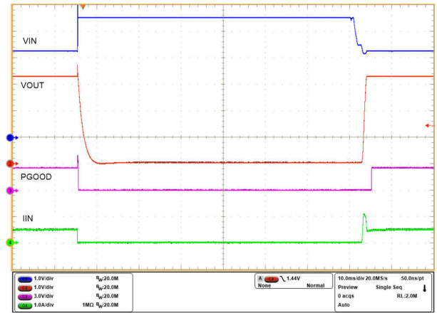
Figure 9-20. Overvoltage Protection Response and Recovery with TPS2598020 Device
