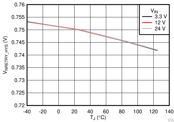
Figure 6-21. NRETRY Oscillator Hysteresis vs Temperature
