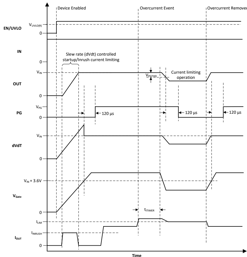
Figure 7-5. Power Good Assertion and De-assertion
