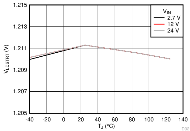
Figure 6-16. LDSTRT Threshold Voltage vs Temperature D021
