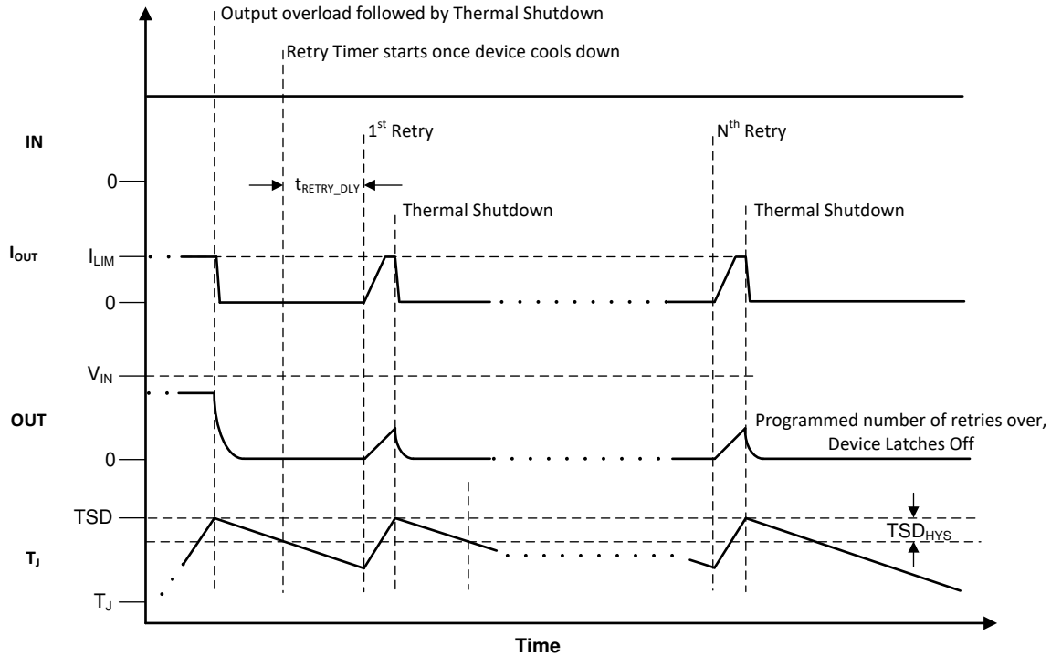
Figure 7-9. Auto-Retry After Fault
