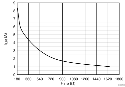
Figure 6-10. Output Current Limit (I LIM ) vs R LIM
