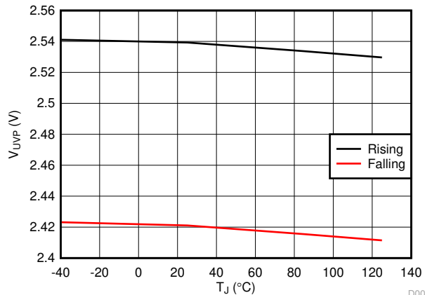
Figure 6-1. Supply UVP Threshold vs Temperature
