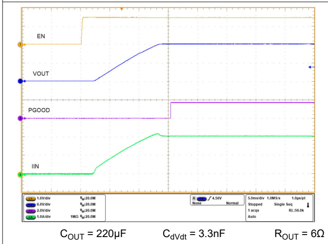
Figure 6-26. Startup With EN Into Resistive Load - dVdt Limited
