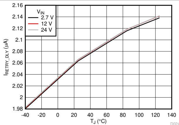
Figure 6-18. RETRY_DLY Bias Current vs Temperature D024
