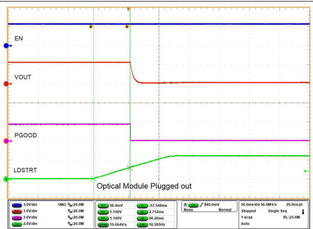
Figure 8-16. Output Voltage Profile When Optical Module is Plugged Out
