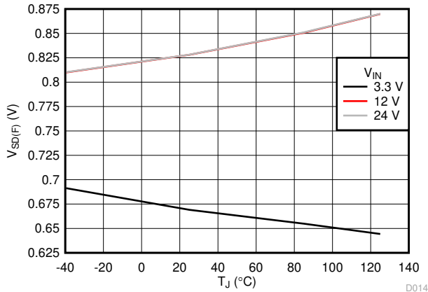
Figure 6-7. EN/UVLO Falling Threshold for Lowest Current Consumption
