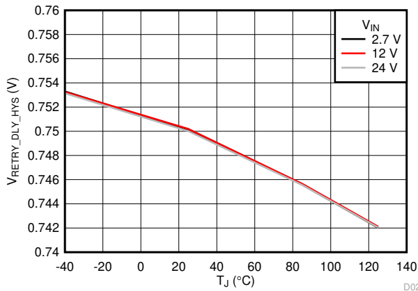
Figure 6-19. RETRY_DLY Oscillator Hysteresis vs Temperature
