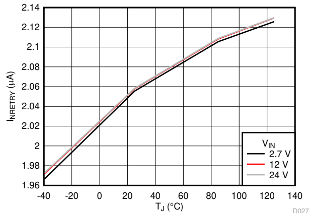
Figure 6-20. NRETRY Bias Current vs Temperature
