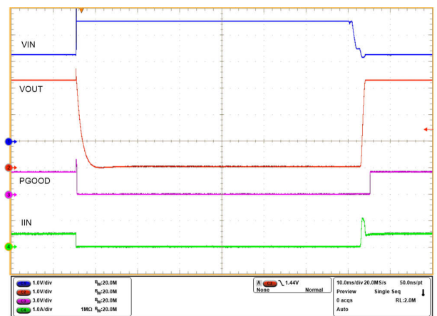
Figure 8-20. Overvoltage Protection Response and Recovery with TPS2598020 Device
