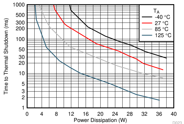
Figure 6-22. Thermal Shutdown Plot - Steady State
