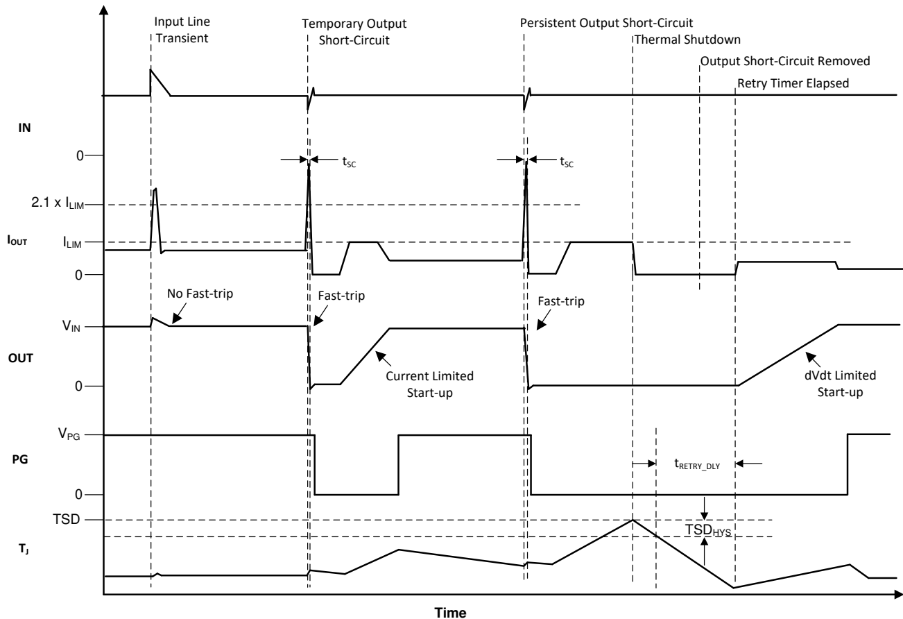
Figure 7-4. Input Line Transient and Output Short-Circuit Response
