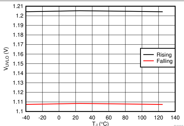
Figure 6-5. EN/UVLO Threshold vs Temperature
