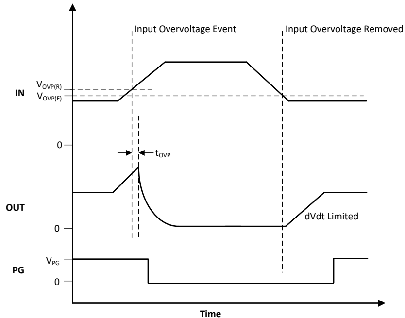
Figure 8-2. Overtoltage Response
