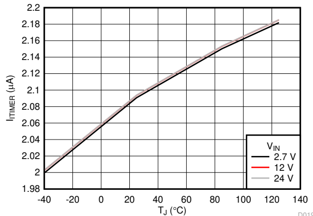
Figure 6-14. ITIMER Discharge Current vs Temperature D019
