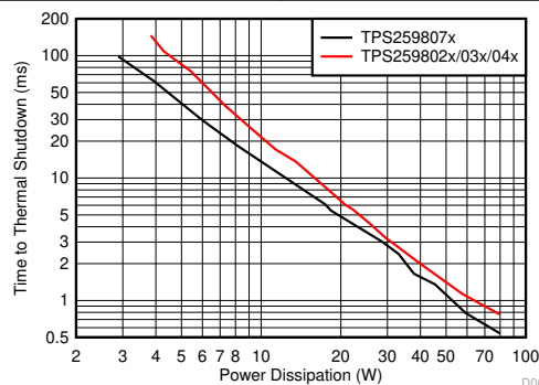
Figure 6-23. Thermal Shutdown Plot - Inrush/Overload
