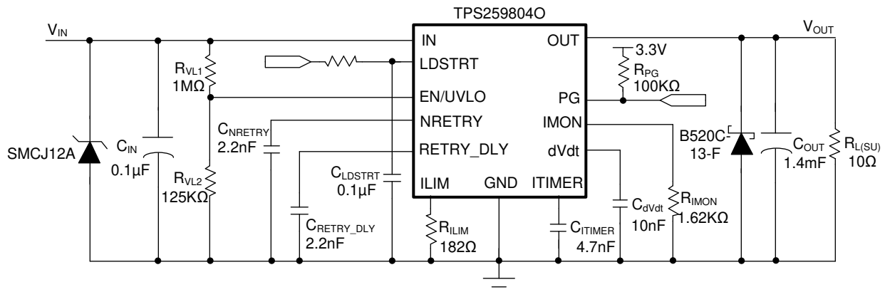
Figure 8-1. Typical Application Schematic - Input Protection for Patient Monitoring System
