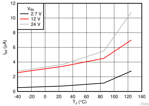
Figure 6-9. Deep Shut-Down Current vs Temperature
