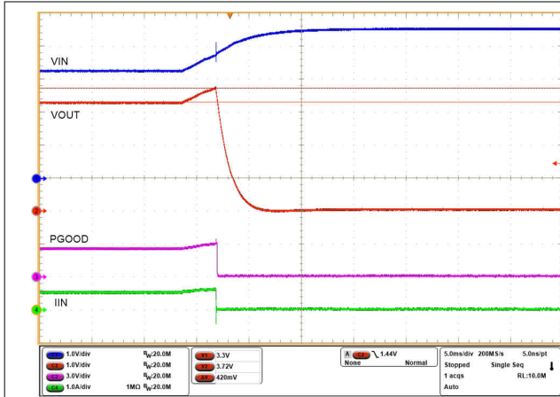
Figure 9-19. Overvoltage Cut-off at 3.7 V with TPS2598020 Device
