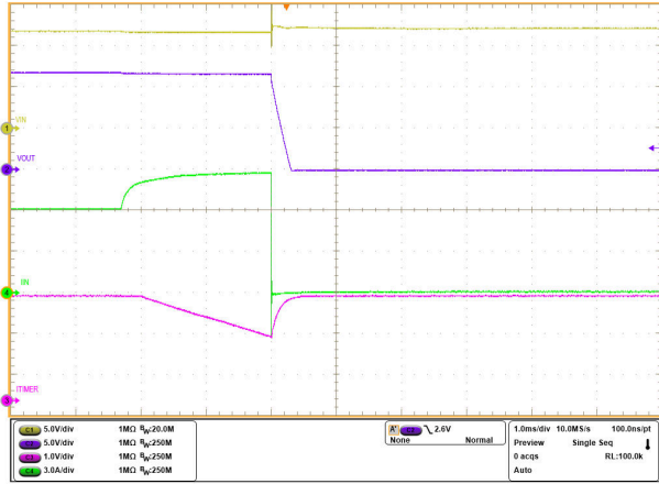
Figure 6-28. Circuit Breaker With Transient Overcurrent Blanking
