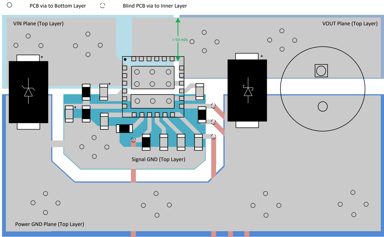
Figure 8-22. TPS25980 Example PCB Layout
