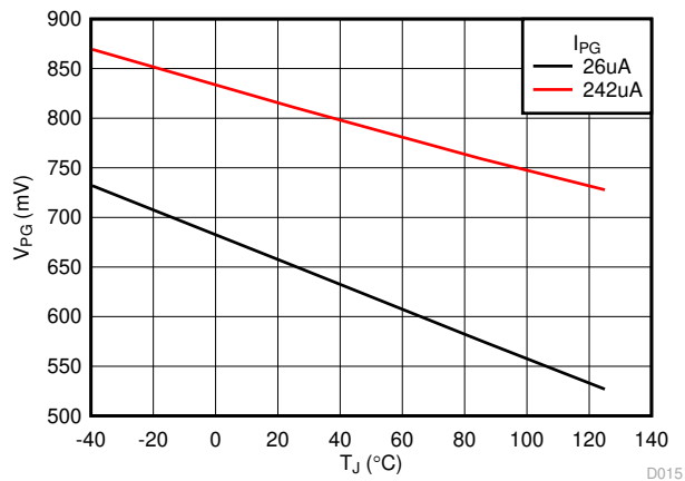
Figure 6-12. Power Good Output Voltage (De-asserted State) vs Temperature
