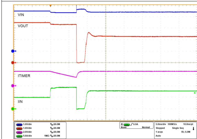
Figure 9-17. Circuit Breaker With Transient Overcurrent Blanking Interval of 6 ms; Device Restarts in Current Limit Mode
