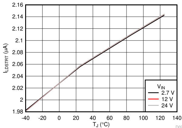
Figure 6-15. LDSTRT Charging Current vs Temperature D020
