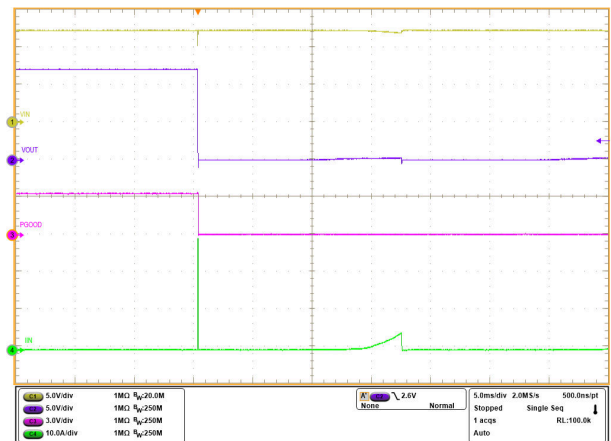
Figure 6-29. Circuit Breaker - Auto-Retry
