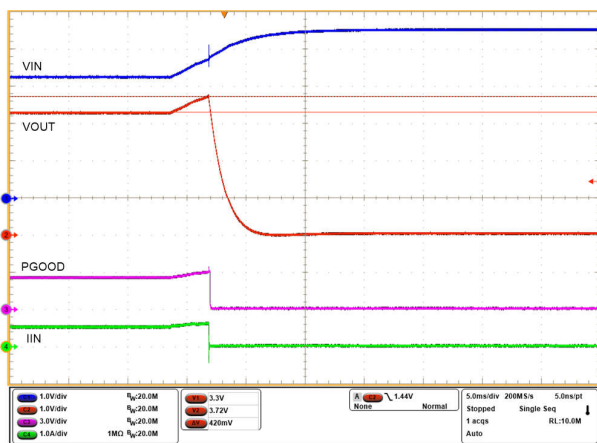
Figure 8-19. Overvoltage Cut-off at 3.7V with TPS2598020 Device
