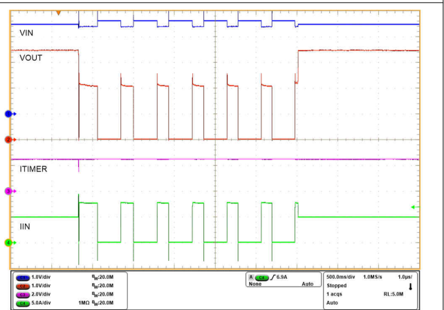
Figure 9-18. Overload Response and Recovery
