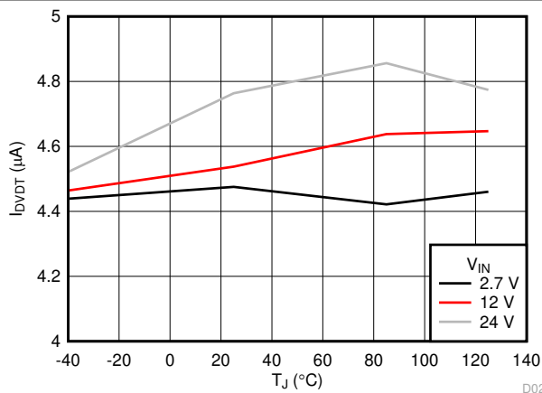
Figure 6-17. DVDT Charging Current vs Temperature D022
