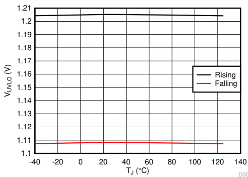
Figure 7-5. EN/UVLO Threshold vs Temperature
