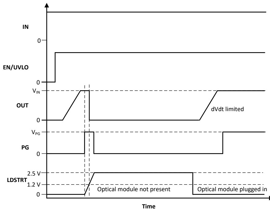
Figure 7-8. Optical Module Plug-In Detection Using LDSTRT
