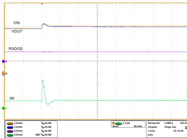
Figure 6-34. Supply Line Transient Immunity - Adjacent Load Hot Unplug
