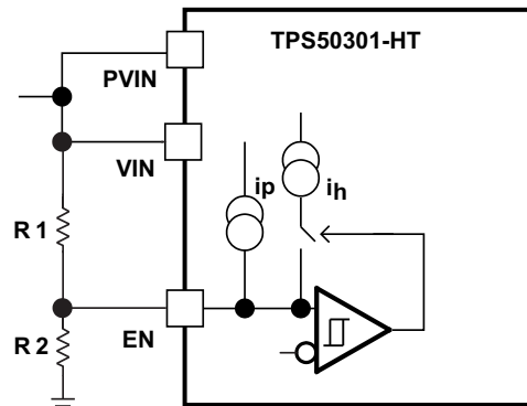
Figure 20. Adjustable VIN and PVIN UVLO
