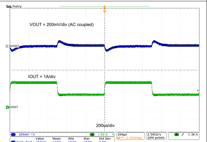
Figure 7-11. TPS542021EVM Load Transient Response, 1A to 2A Load Step
