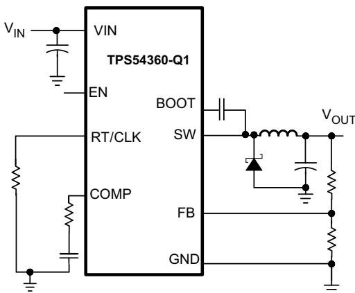
Simplified Schematic
