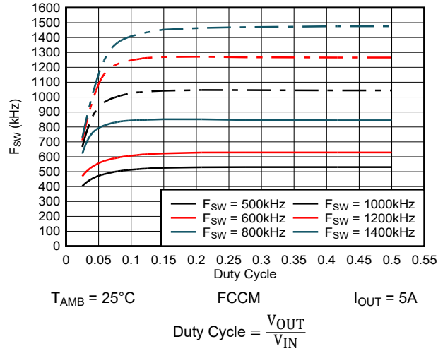
Figure 6-13. Switching Frequency vs Duty Cycle
