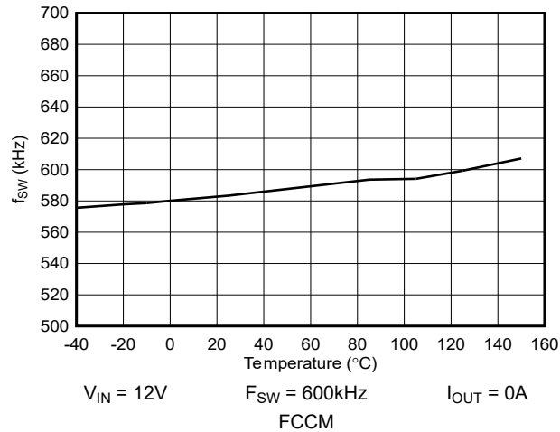
Figure 6-15. Switching Frequency vs Junction Temperature
