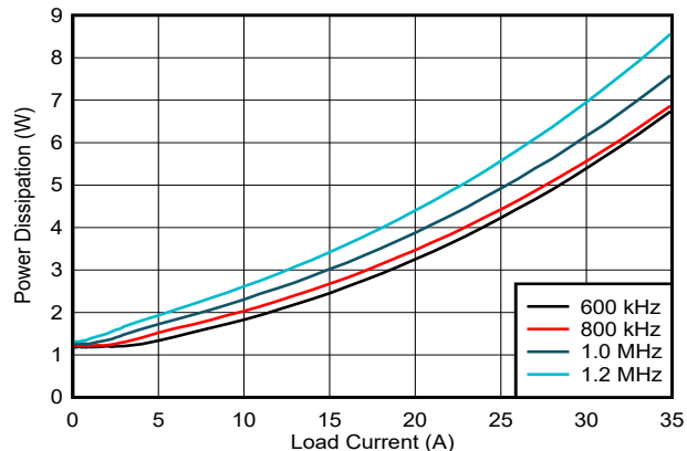
Figure 8-3. Power Dissipation, FCCM, Internal LDO
