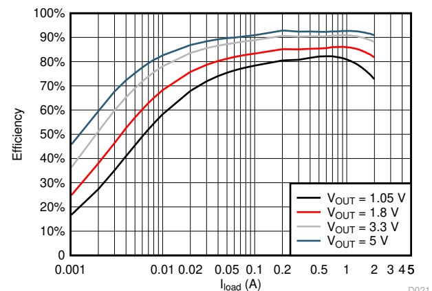
TPS562201 Efficiency
