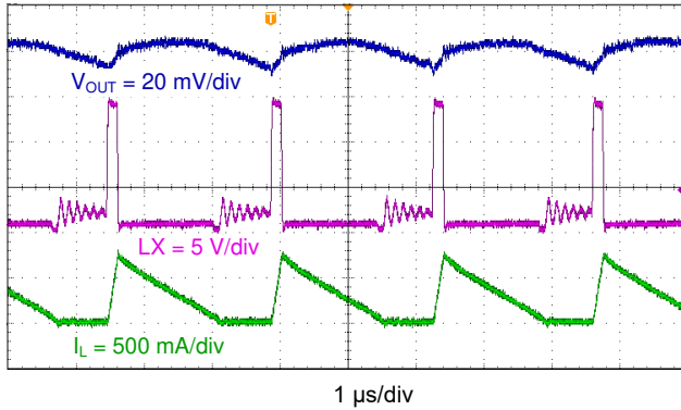
Figure 7-8. TPS563201 Output Voltage Ripple, I_{out} = 0.25 A
