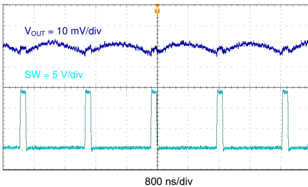
Figure 7-10. TPS563208 Output Voltage Ripple, I_{OUT} = 0 A
