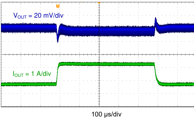
Figure 7-12. TPS563201 Transient Response, 0.75 to 2.25 A
